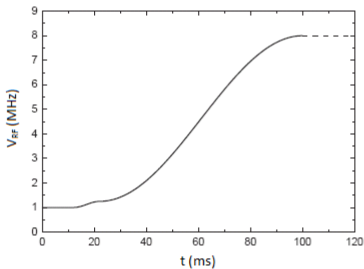
Figure 1: RF “Ramp” Used to Trap Supercooled Atoms
