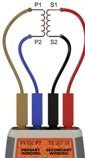
Figure 2.2 TPT9000 connections to a test transformer
