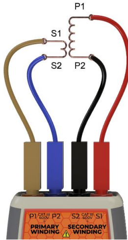
Figure 2.3 TPT9000 connections to a test transformer with a high impedance Primary winding
